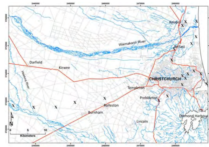
Figure 8. Distribution of I_{ESI-2007}=X for the September 4 th earthquake based on surface faulting, the spatial distribution and severity of liquefaction, lateral spreading and ground subsidence.
