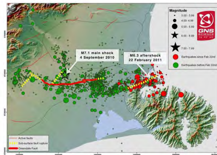
Figure 1. Earthquake sequences of September 4th, 2010 and February 22nd, 2011 and the fault zones that were activated (GNS 2011).
