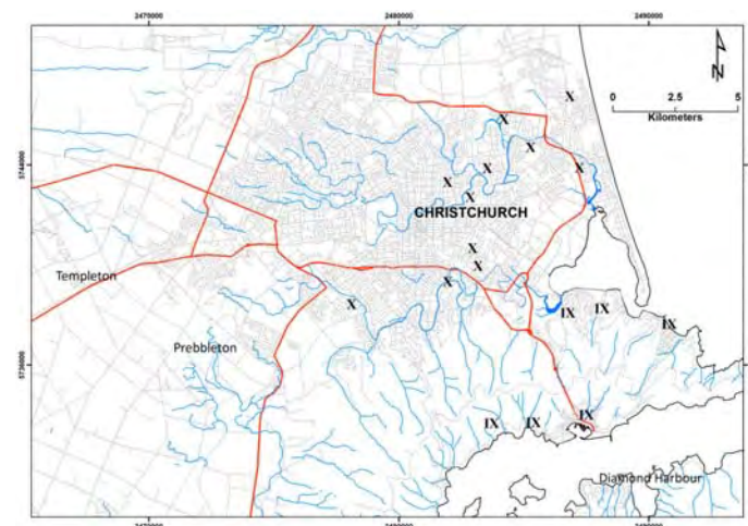
Figure 9. Distribution of I_{ESI-2007}=X and I_{ESI-2007}=IX for the February 22 nd earthquake based on the severity and spatial distribution of liquefaction, lateral spreading, ground subsidence and volume of mass movements.
