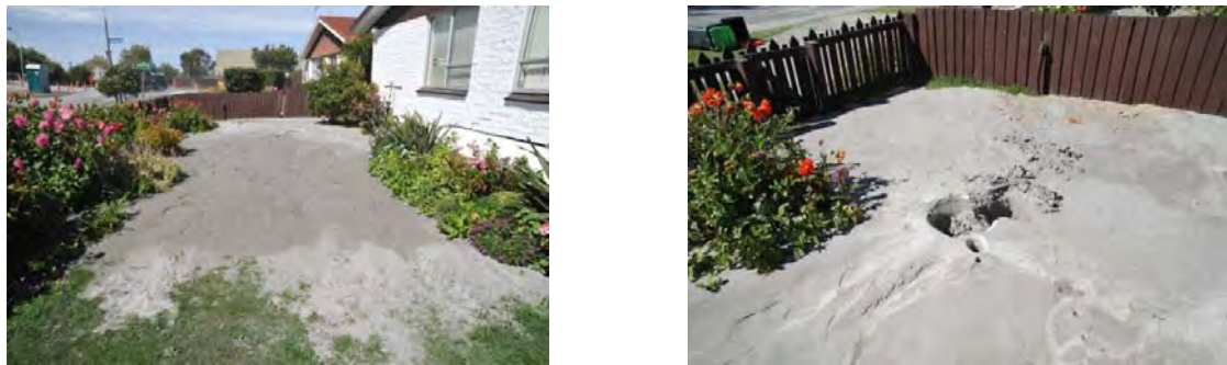
Figure 6. Views of liquefaction phenomena in the area of Christchurch after the earthquake of February 22, 2011.
