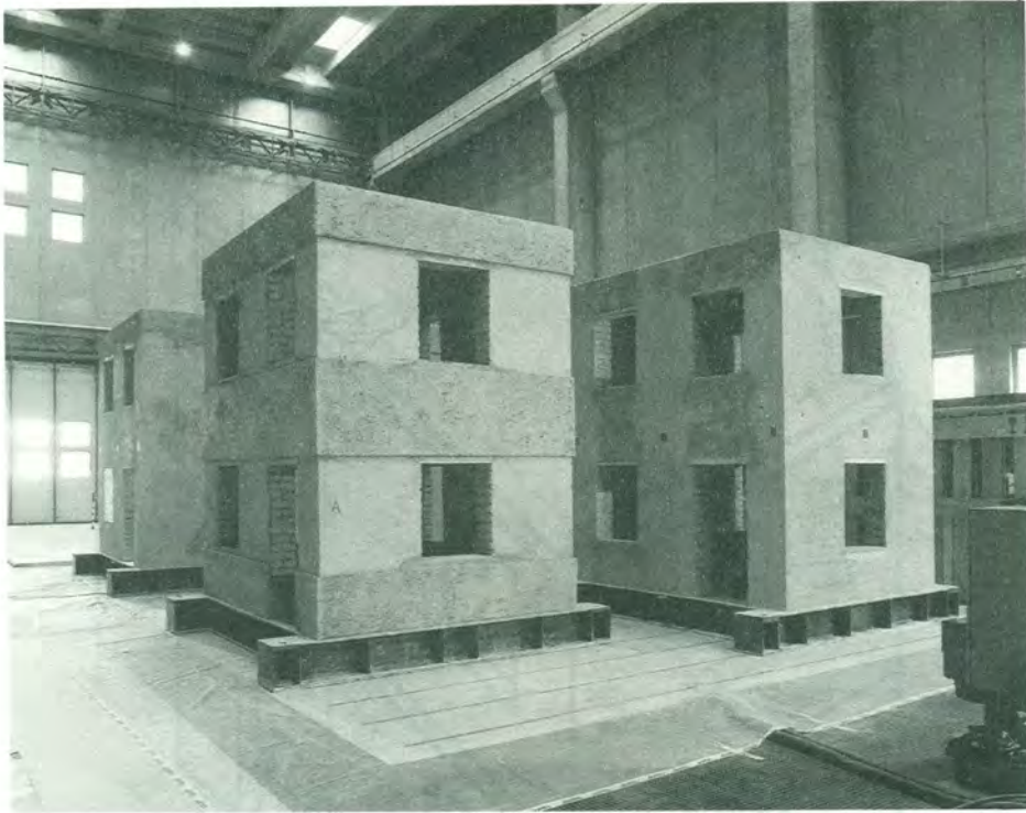
Figure 2. Three ISMES buildings (brick masonry). The central building is strengthened by rb
