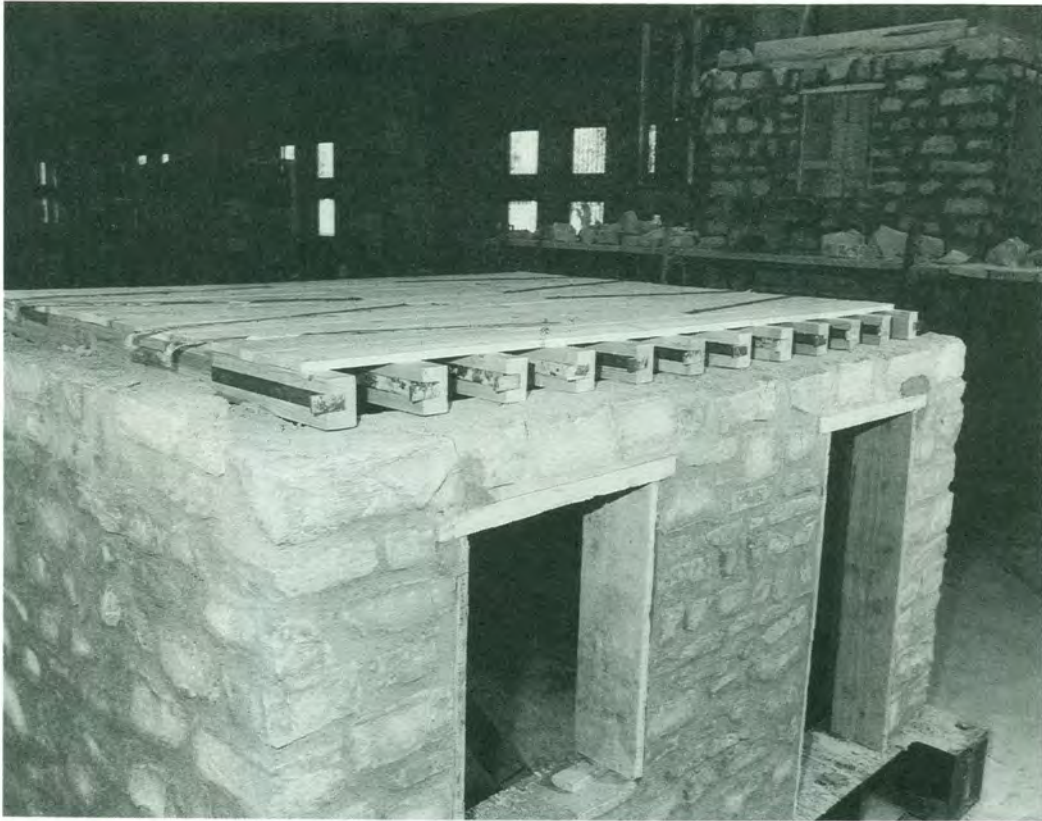
Figure 4. Improvement of the connections of slabs to walls by steel anchors (sc)
